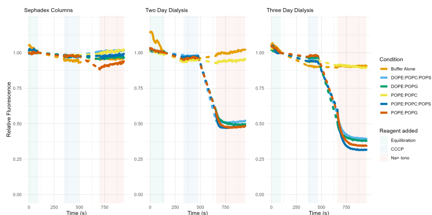
Figure 3.12.: The \text{Na}^+ flux assay reliably measures flux through empty vesicles composed of a variety of lipid mixes. Lipid mixes (colors) were tested for the ability to form vesicles as measured by the flux assay. Three different methods of forming vesicles were tested (facets).
