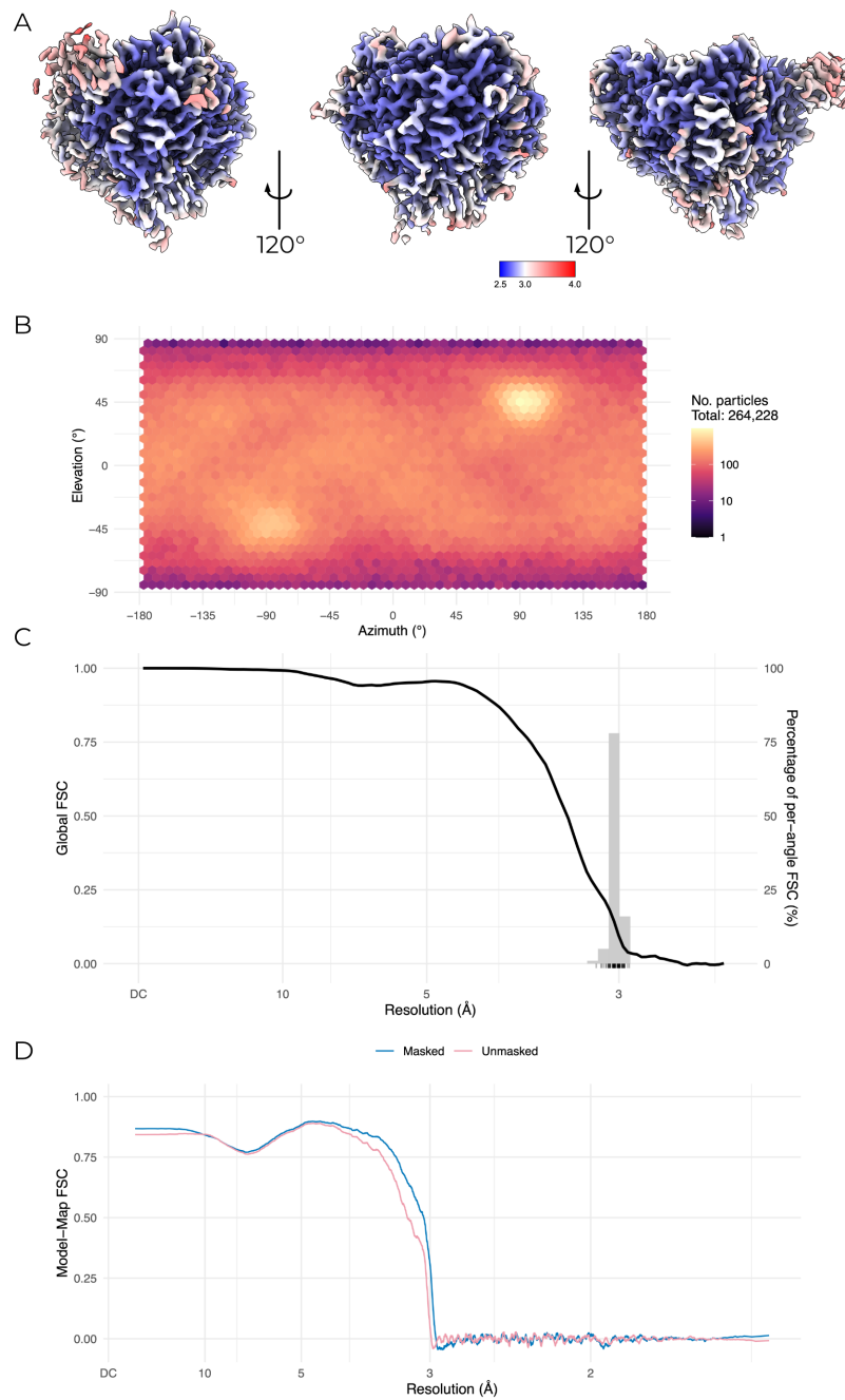
Figure D.6.: Validation of trypsin-cleaved mouse map and model.
