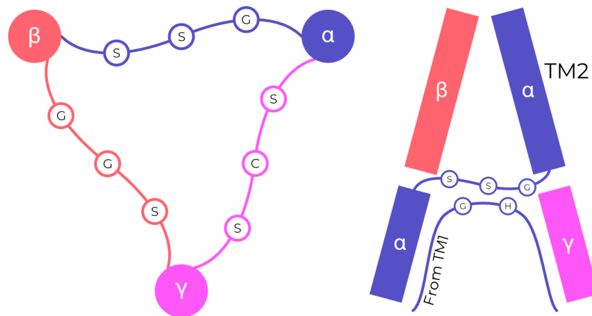
Figure 2.10.: A cartoon of ENaC’s selectivity filter. Left: a top-down view of the domain swap loop. Right: a schematic illustration of \alpha TM2 breaking and completing \beta TM2. The concept of a domain swap is supported by structures of other ENaC/DEG channels and studies of ENaC mutants.
