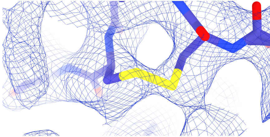
Figure 5.1.: The human CKO/DEG map surrounding the disulfide between \alpha C479 and \alpha C394.
