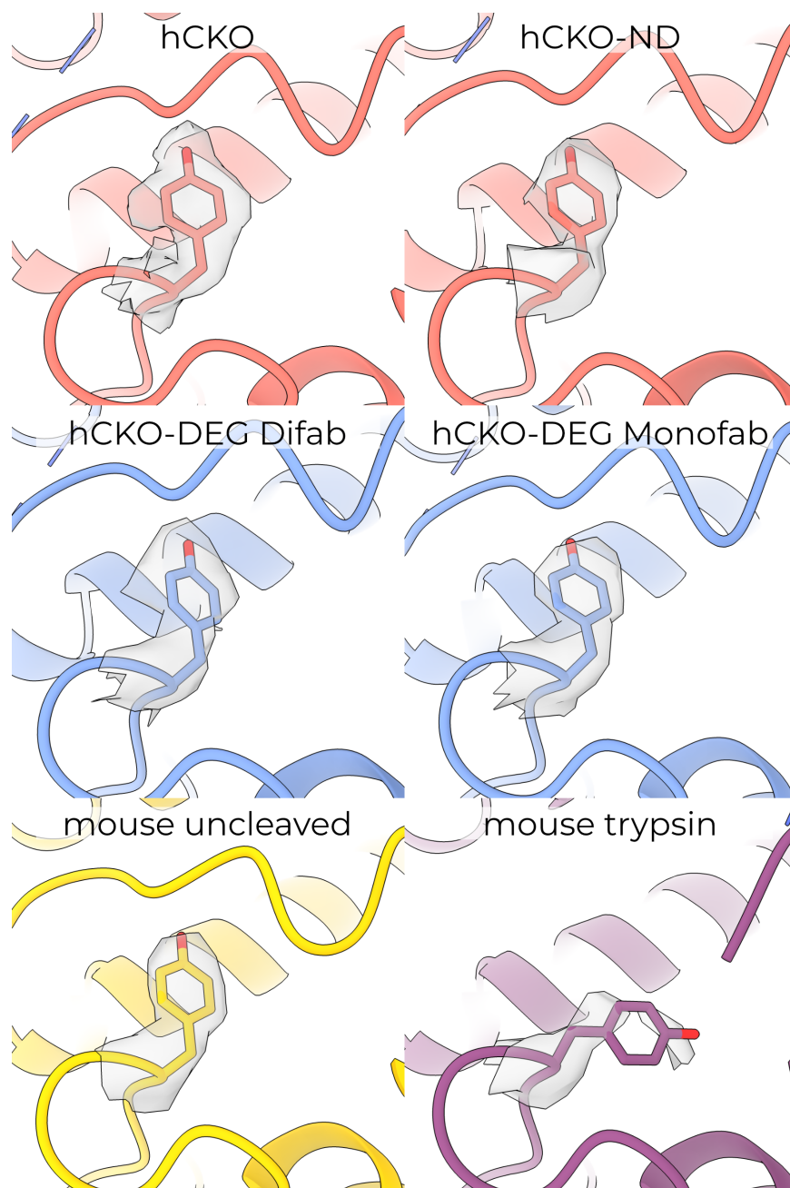
Figure 4.6.: CryoEM map potential for strained \gamma ENaC tyrosine for all maps/models. The maps are masked around the residue of interest.
