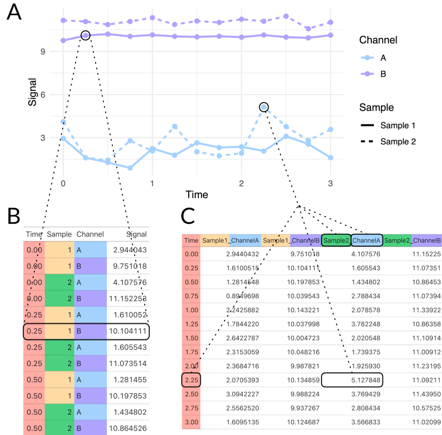
Figure E.2.: Data formats saved by Appia and available for user download. Traces made up of individual samples (A) are represented as a single row in the long format (B). The wide format (C) instead represents the independent variable with its own column (Time, red), the response variable with the table body (Signal, white), and all other variables in column headers (various colors).
