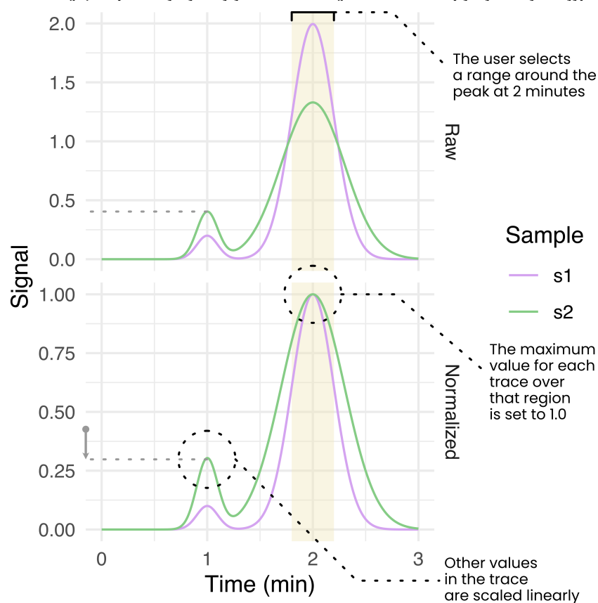
Figure E.3.: Appia's normalization process. A user-selected region is used to linearly scale all traces such that their maximum value over that region is 1.
