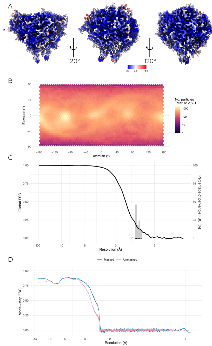
Figure D.1.: Validation of human CKO map and model.
