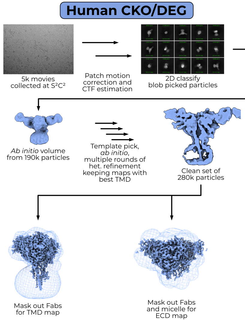
Figure C.3.: Human CKO/DEG Difab pipeline.
