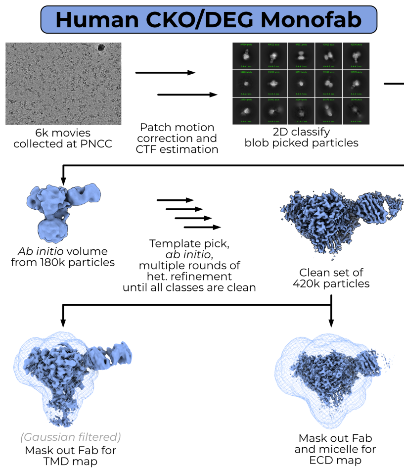
Figure C.4.: Human CKO/DEG Monofab pipeline.
