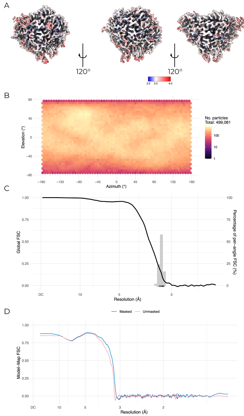
Figure D.5.: Validation of mouse uncleaved map and model.
