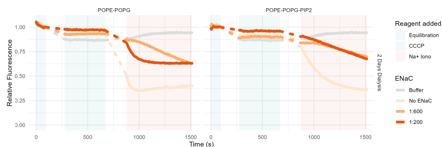
Figure 3.13.: The flux assay was performed with two lipid mixes (facets). In addition to the buffer control (grey), three ENaC:lipid ratios were tested: no ENaC, 1:600, and 1:200 (increasing color saturation). None of these show a decrease in fluorescence with addition of CCCP, indicating that there was no \text{Na}^+ flux in any mixture.
