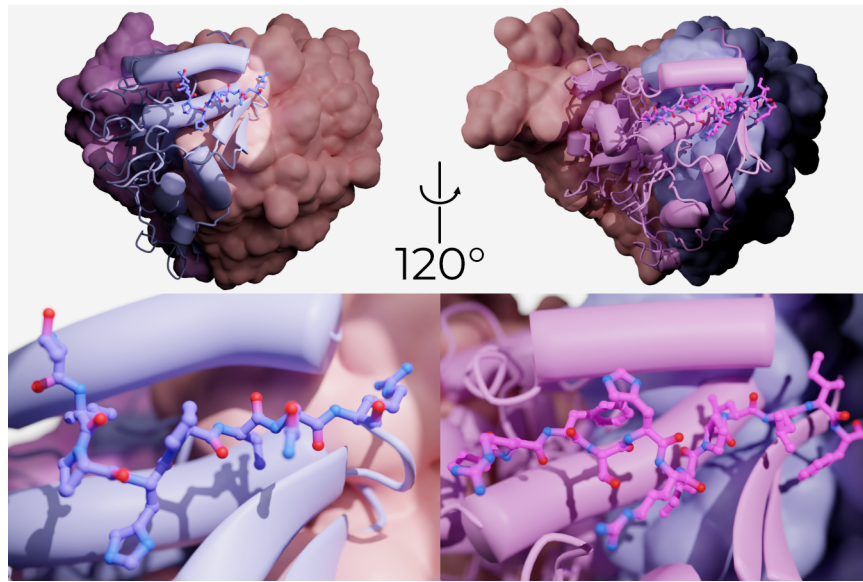
Figure 2.9.: The inhibitory peptides of the \alpha (left) and \gamma subunits. PDB: 6WTH.
