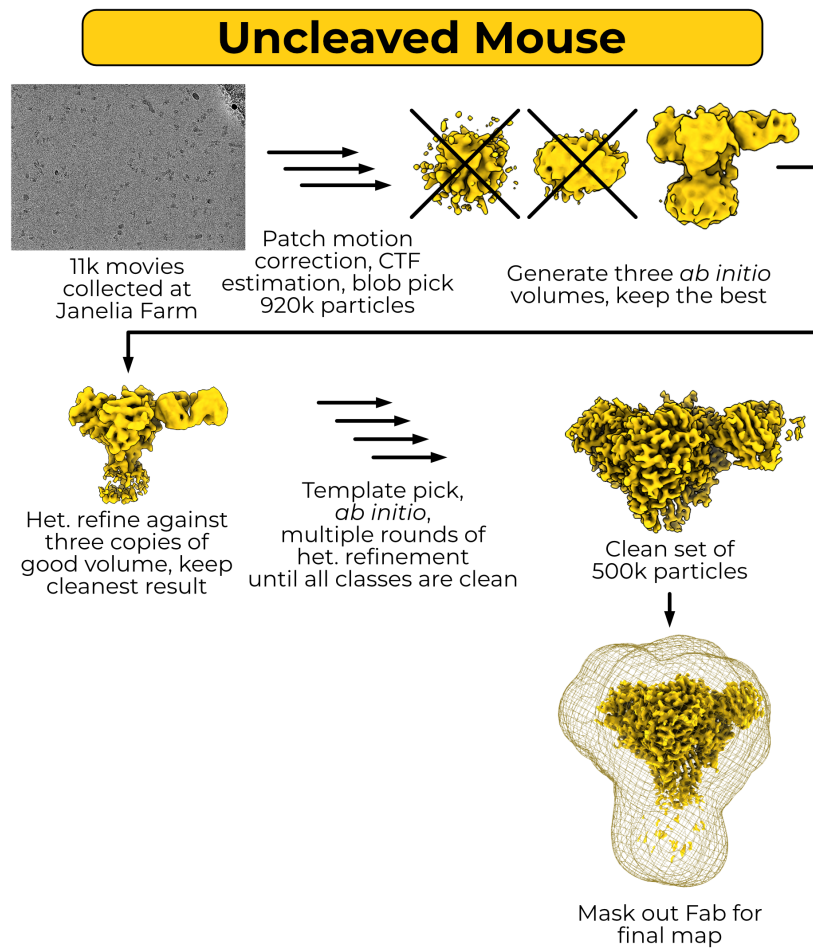
Figure C.5.: Mouse uncleaved pipeline.
