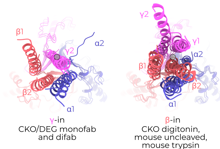
Figure 3.6.: The ENaC transmembrane domain adopts two conformations. TMDs of all six ENaC models separated by TM conformation, viewed from the intracellular side. Models are in the same position and at the same scale in each image, so positions are directly comparable. A grayed circle is added in the same position to aid comparison between panels.
