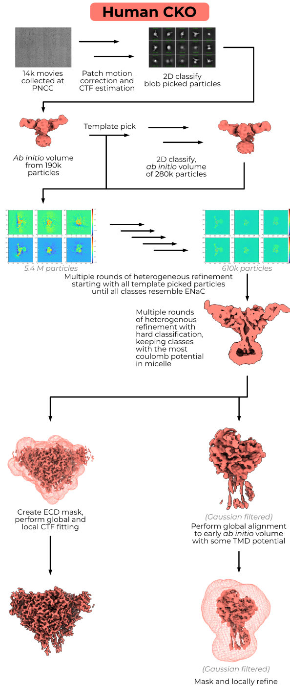
Figure C.1.: Human CKO processing pipeline. The TMD volumes are gaussian filtered to reduce noise.
