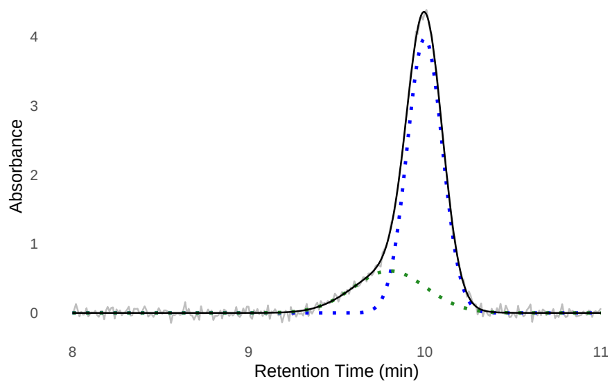
Figure E.5.: Fitted values plotted atop data. Bound and unbound are green and blue respectively, with the additive model in black.
