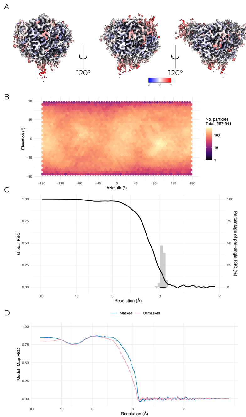
Figure D.2.: Validation of human CKO-DEG map and model.
