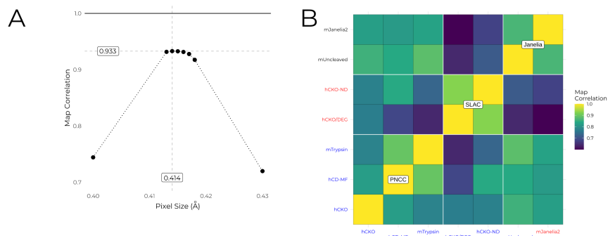
Figure A.1.: S^2C^2 pixel sizes seem miscalibrated. A : Scaling the nominal pixel size for human CKO/DEG dramatically increases the correlation with human CKO digitonin. B : Correlation coefficients for all maps. Maps were aligned prior to taking correlation coefficients. Abbreviated as follows: hCKO: human CKO; hCD-MF: human CKO/DEG monofab; mTrypsin: trypsin-cleaved mouse; hCKO/DEG: human CKO/DEG difab; hCKO-ND: human CKO nanodisc; mUncleaved: mouse uncleaved; mJanelia2: a second uncleaved mouse dataset collected at Janelia, but not presented here.
