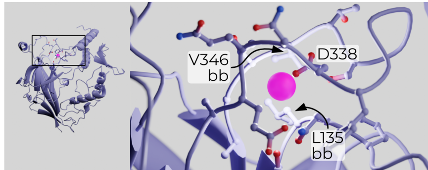
Figure 2.12.: The acidic pocket of \alpha ENaC. Residues close enough to bind the putative \text{Na}^+ ion are labeled. A residue label including “bb” indicates that the carbonyl oxygen of the main chain binds the ion. PDB: 6WTH.
