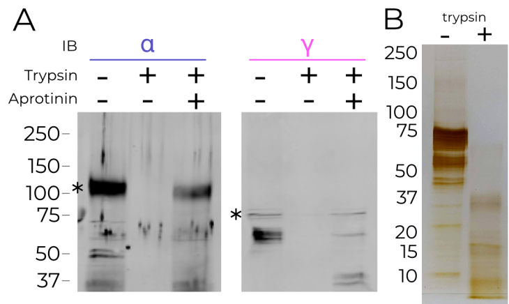
Figure 4.2.: Purified ENaC is cleaved by trypsin. A: Western blot for \alpha (left) and \gamma (right) ENaC. Purified mouse protein was treated with trypsin and aprotinin as indicated. Bands corresponding to full-length subunits are marked with an asterisk. B: Silver stain of material with and without trypsin treatment. Material for silver stain and western blot is from different expressions and purifications.
