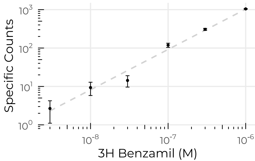
Figure 3.9.: An example of SPA, in this case of CKO/DEG nanodiscs. Note that although the background counts have been subtracted, the relationship between ligand and counts is still linear.
