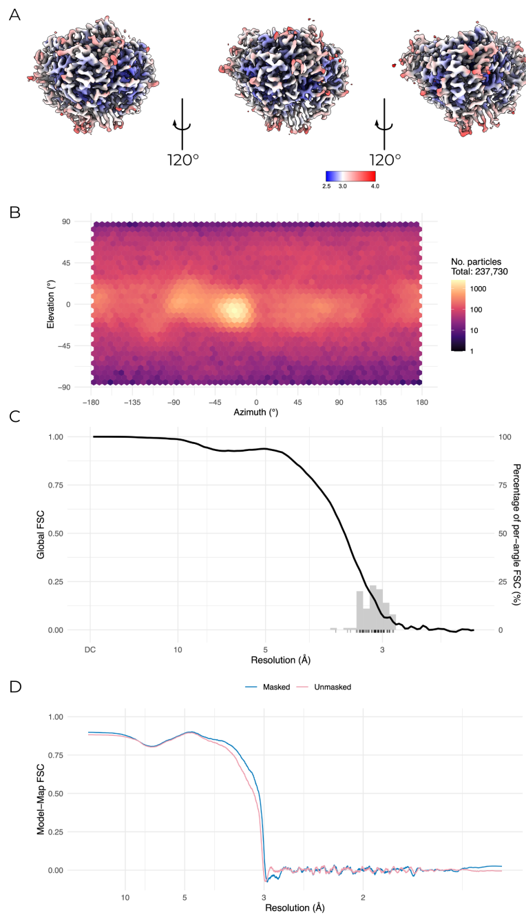
Figure D.4.: Validation of human CKO nanodisc map and model.
