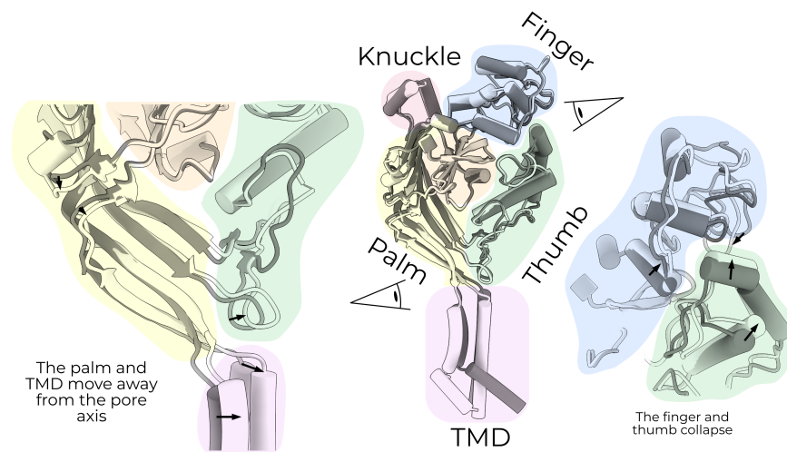
Figure 2.3.: A diagram of ASIC's gating conformational changes. When resting ASIC (grey) are protonated (white), the finger and thumb collapse (right). This movement is coordinated with the movement of the lower palm and TMD away from the pore axis, which opens the extracellular fenestration (left).
