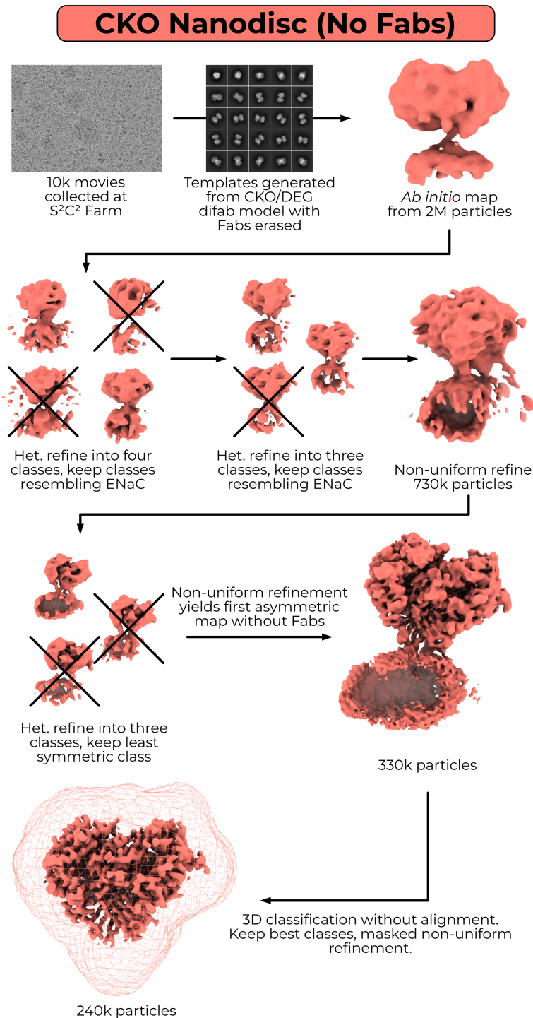
Figure C.2.: Human CKO nanodisc pipeline. Masks are contoured to 0.5. Note that the CKO/DEG map was provided in the form of low-pass filtered templates for particle pick 161 , but never to an alignment.
