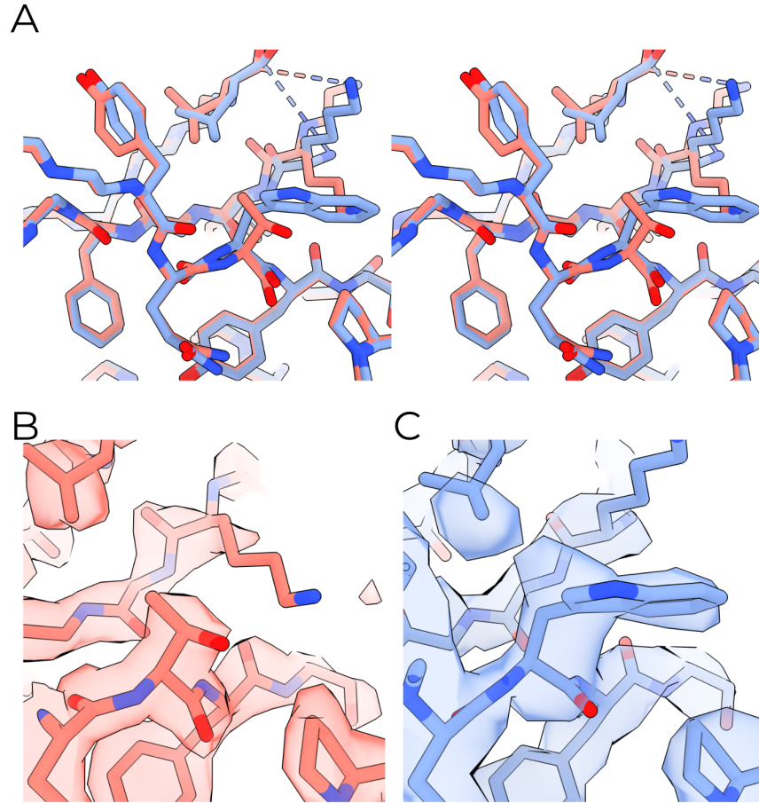
Figure 3.8.: The \alpha T240W mutation does not modify ECD conformation. A : Stereo view of the GRIP domain near \alpha T240. Red: CKO, blue: CKO/DEG monofab. B and C : CryoEM map potential surrounding \alpha 240 in CKO and CKO/DEG monofab, respectively.
