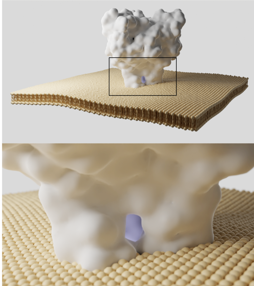
Figure 2.4.: The fenestration in ASIC. Membrane is for illustration purposes only and is not based on actual structural data. PDB: 4NTW.
