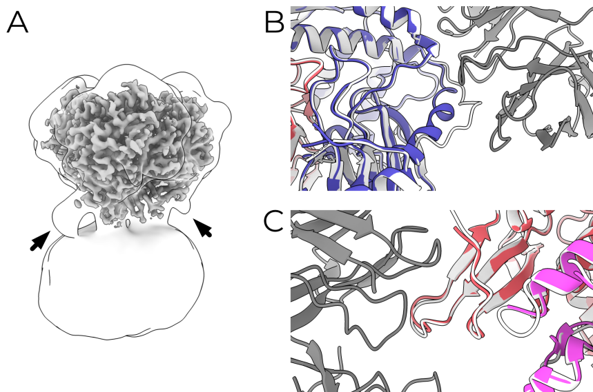
Figure 4.7.: Fab binding induces only minor changes in the extracellular domain of ENaC. A: Human CKO/DEG map. A low-pass filtered map is outlined to show pseudosymmetry-breaking glycosylation sites (arrows). B: the \alpha subunit, C: the \beta subunit. Human CKO nanodisc model is colored by subunit, the human CKO/DEG ENaC is white, and human CKO/DEG Fabs are grey.
