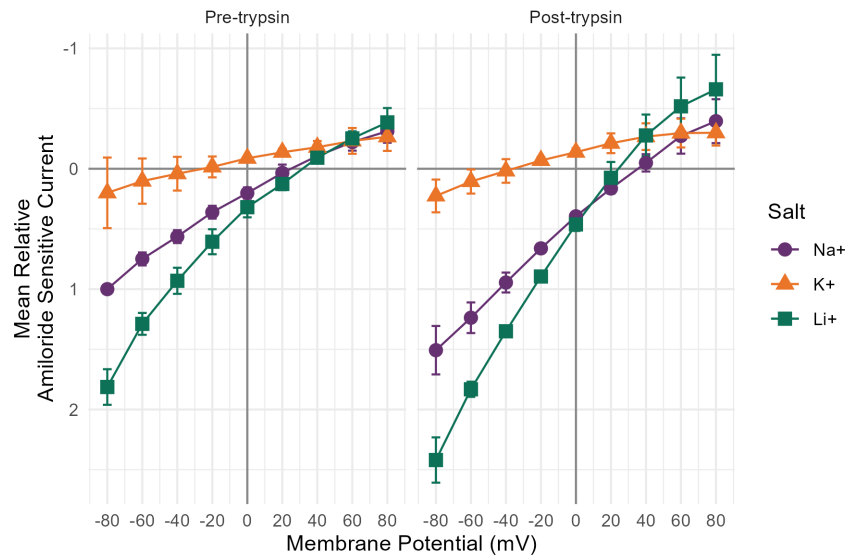
Figure 4.11.: I/V curves for human CKO and CKO/DEG channels. Values are normalized per-cell to the inward current at -80 mV before trypsin treatment. Cells were treated with trypsin for five minutes before being re-recorded. Each point is the average of three cells. Error bars represent +/- one standard deviation.
