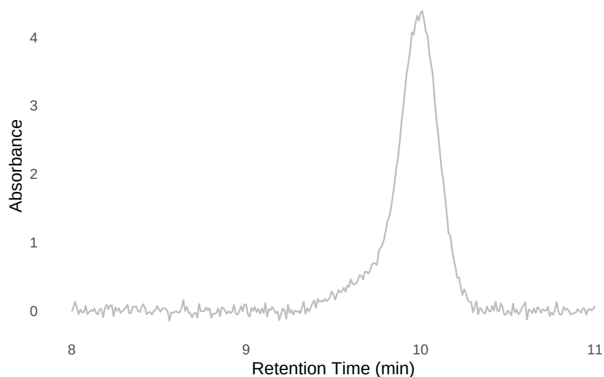
Figure E.4.: Example data of a mixture between a protein and a Fab.
