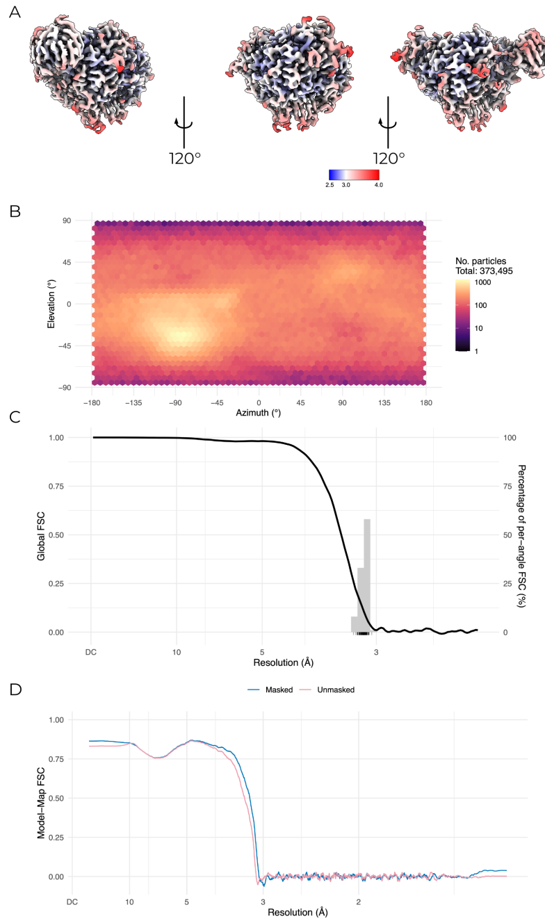
Figure D.3.: Validation of human CKO-DEG monofab map and model.
