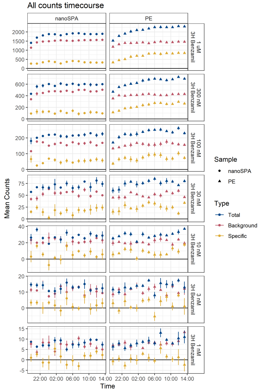
Figure B.10.: Comparison of nanoSPA and Perkin Elmer (PE) beads. In this context, “background” and “total” differ only in that “background” does not have any detergent added and “total” does. Note that nanoSPA beads quickly level off to a steady signal while PE beads increase for several hours. Note also that “specific” counts, which should be zero in all cases, are lower in nanoSPA beads than PE. Bars represent the standard error of the mean for three replicates, but are too small to see in the higher-concentration plots.
