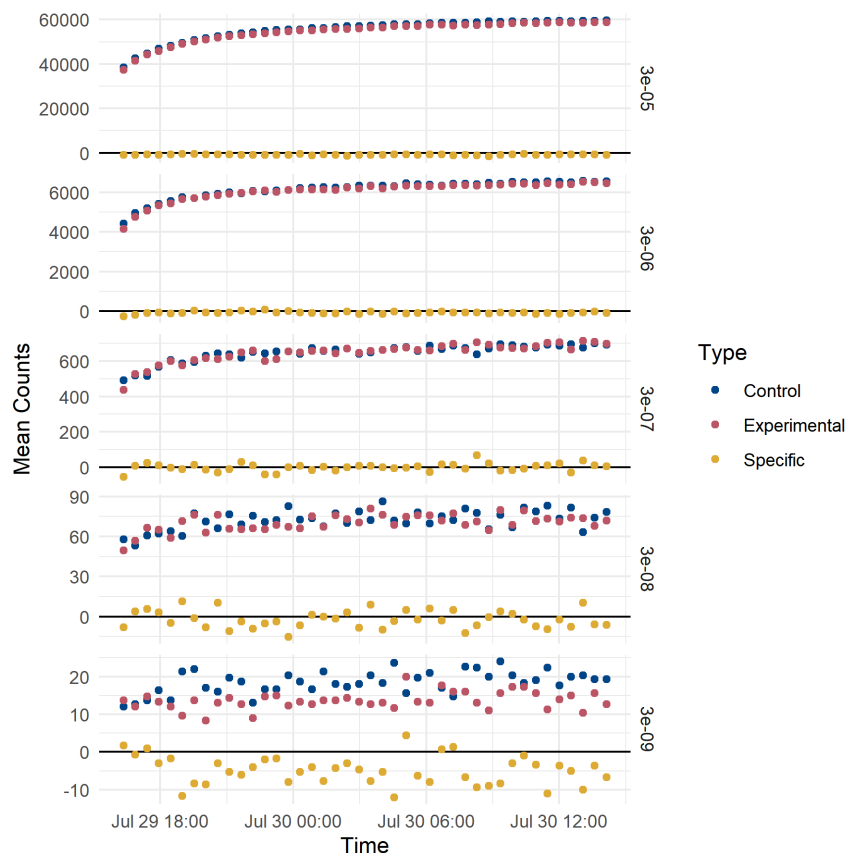
Figure B.8.: The plate is re-recorded approximately every 10 minutes. Note that high ligand concentrations (upper facets) maintain a steady signal, while low ligand concentrations (lower facets) are too noisy to reliably determine. Thus, datasets recorded only 10 minutes apart might show dramatically different Specific (Experimental - Control) counts for low concentrations, which would significantly affect fitted K_d values. Note, also, that despite their stability, specific counts at high ligand concentrations are almost entirely negative.
